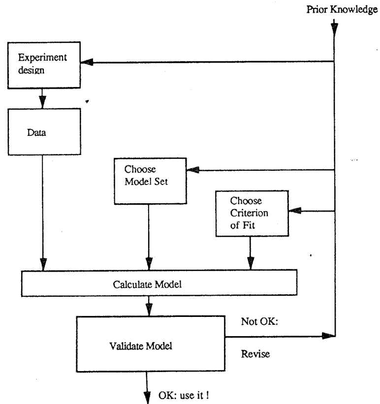
Figure 2: The System Identification Loop. Ljung (1987, p. 9).
