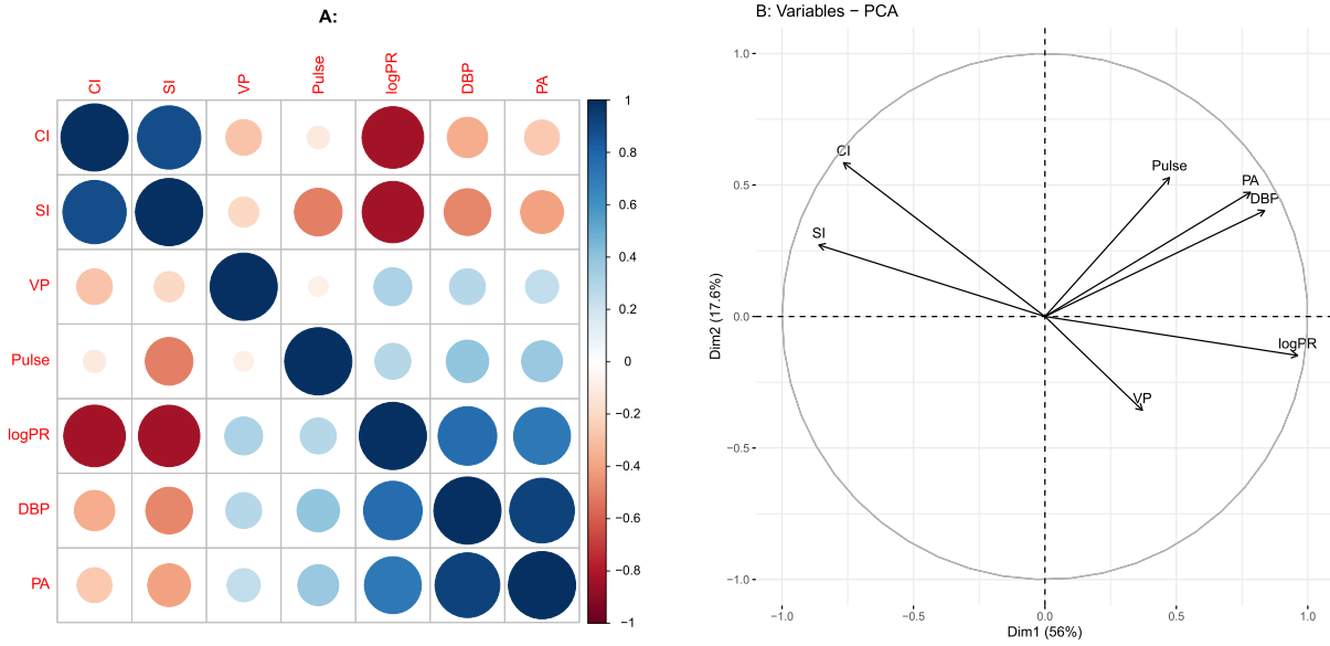
Figure 1. Displays of the correlation matrix of the Heart attack data obtained in R by using the corrplot , FactoMineR , and factoextra packages. A: Colored tabular display or corrogram. B: Correlation circle or correlation biplot. See Section 2 for the abbreviations of the names of the variables.
