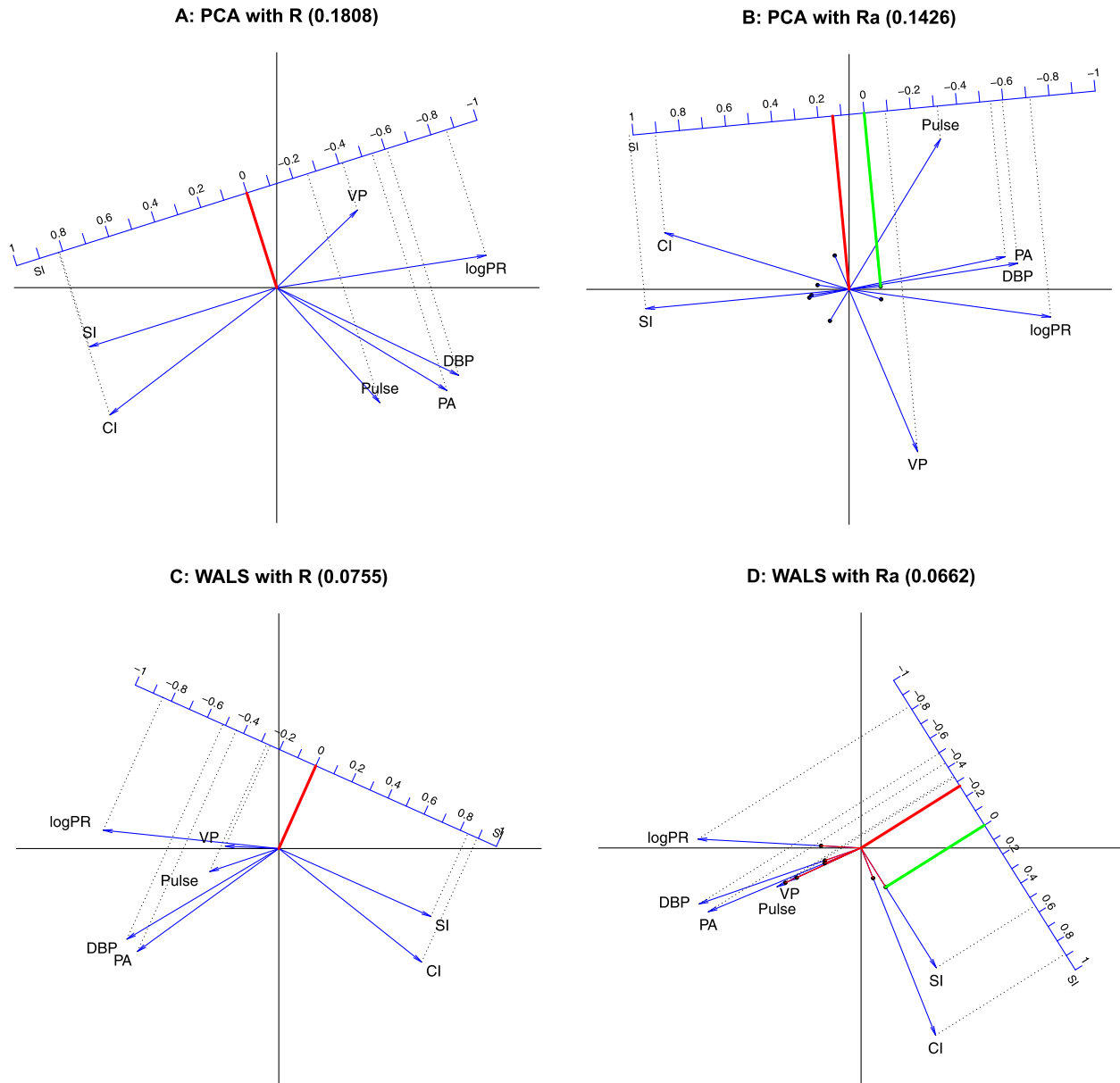
Figure 3. Adjustment of the correlation matrix. All biplots have a calibrated correlation scale for SI . A: PCA biplot; B: PCA biplot using the \delta adjustment; C: WALS biplot; D: WALS biplot using the \delta adjustment. The interpretation of the biplot origin is shown by its projection (in red) onto the calibrated scale. Black dots on biplot vectors correspond to zero correlation for the corresponding variable. The interpretation of the black dot for SI is shown by its projection (in green) onto the calibrated scale. For positive \delta , biplot vectors are extended beyond the biplot origin toward their zero point. For negative \delta , tails of biplot vectors are colored in red for the negative part of the correlation scale.
