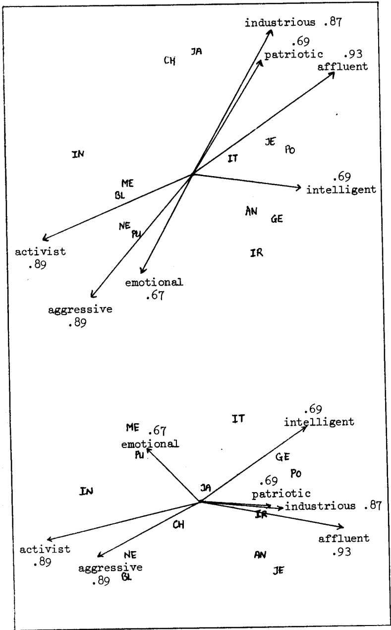
figure 26. Three-dimensional solution for Funk e.a. (first dimension horizontal, second vertical above, third vertical below). Deviation scores, table 12.
