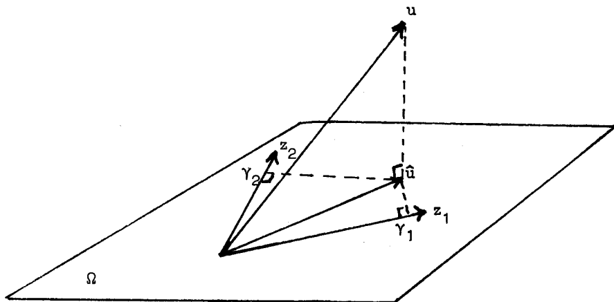
figure 24. Least squares linear regression.
