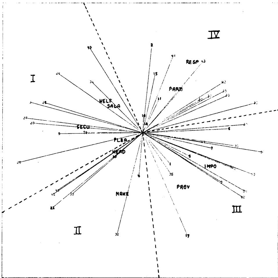
figure 15. Job satisfaction data in deviation from column means (MDPREF, first 2 out of 8, expl.var. 51%).
