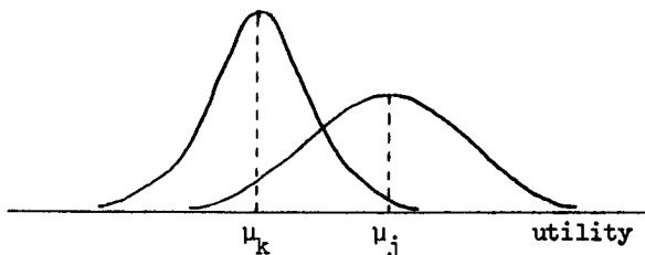
figure 2. Marginal utility distributions ('discriminal processes') for j and k.
