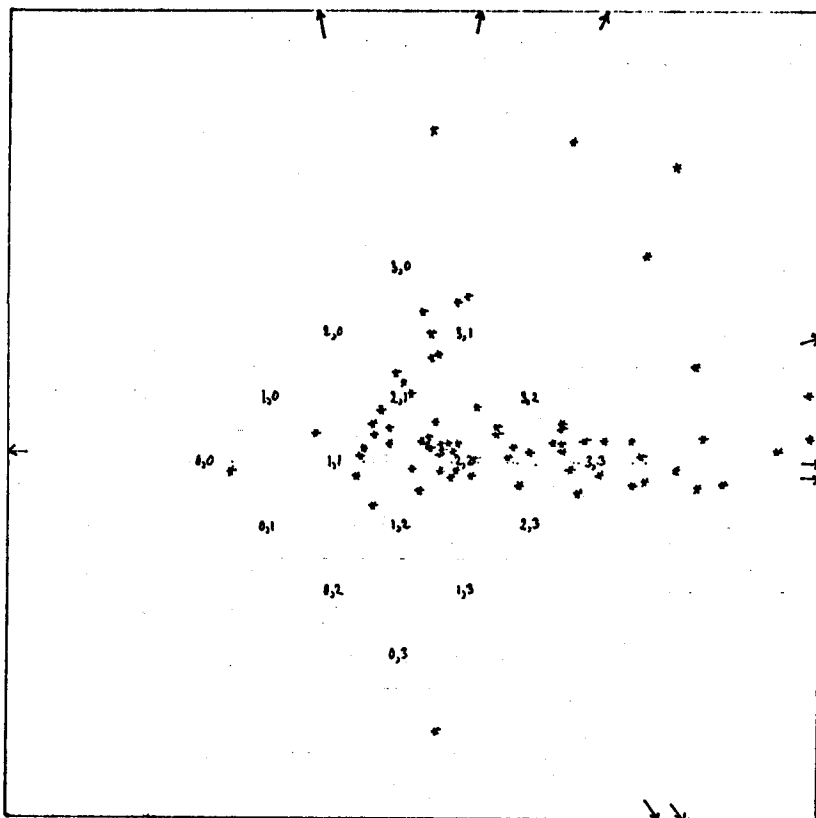
figure 27. Ideal points of Delbeke subjects in the a priori defined family composition space.
