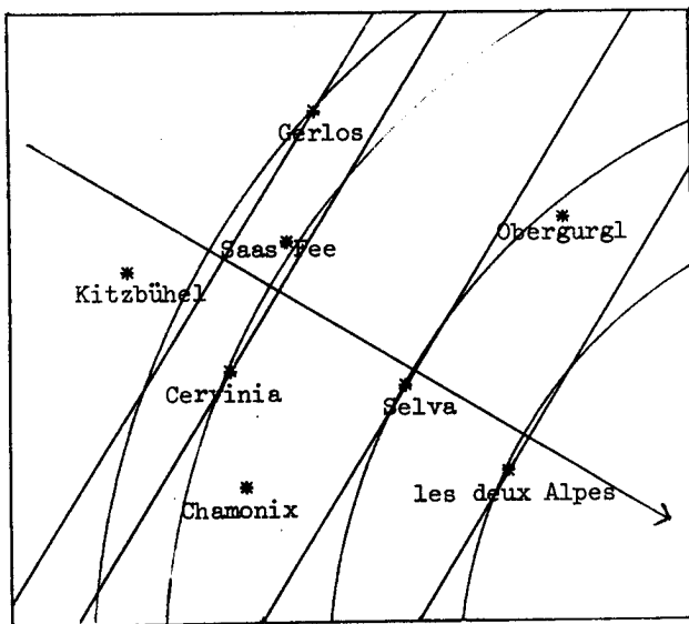
figure 17. Equivalence of circular and straight isochrests when subject point moves outwards.
