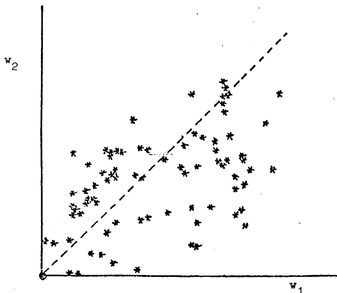
figure 28. Weights for the dimensions in the PREFMAP-phase 2 solution for the Delbeke data.
