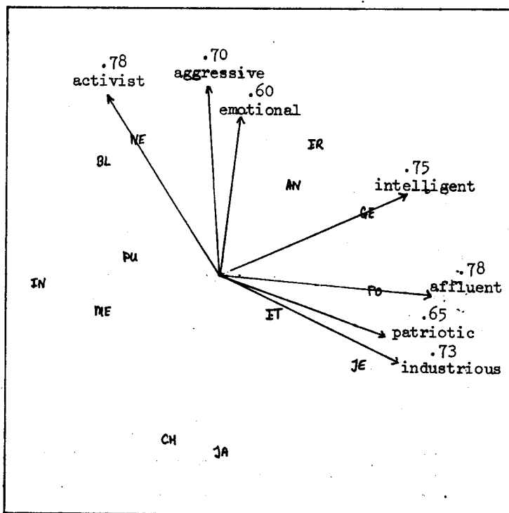
figure 25. Cognitive map of ethnic groups with seven attribute vectors.
