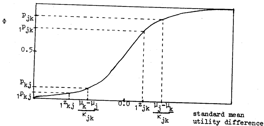
figure 4. The effect of a threshold parameter.
