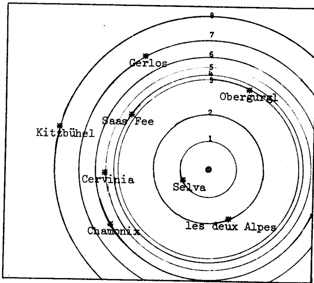
figure 16. Wintersport map with circular isochrests.
