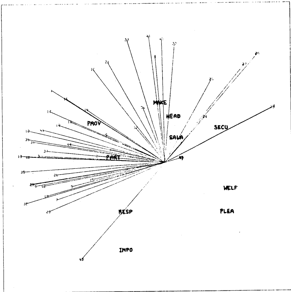
figure 14. First two dimensions of eight-dimensional MDPREF solution for job satisfaction data.
