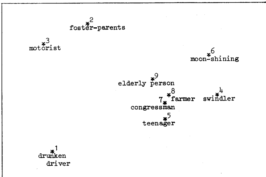
figure 7. Cognitive map obtained for the immorality judgments in table 5 ( L(X,\mu) = 0.0511 ).
