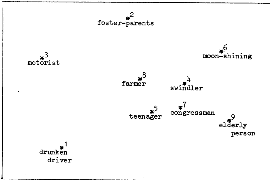
figure 8. Cognitive map obtained from Sjöberg's estimates of the comparatal dispersions (metric stress = .17244).
