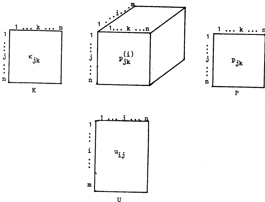
figure 1. Central three-way datablock with three derived matrices
