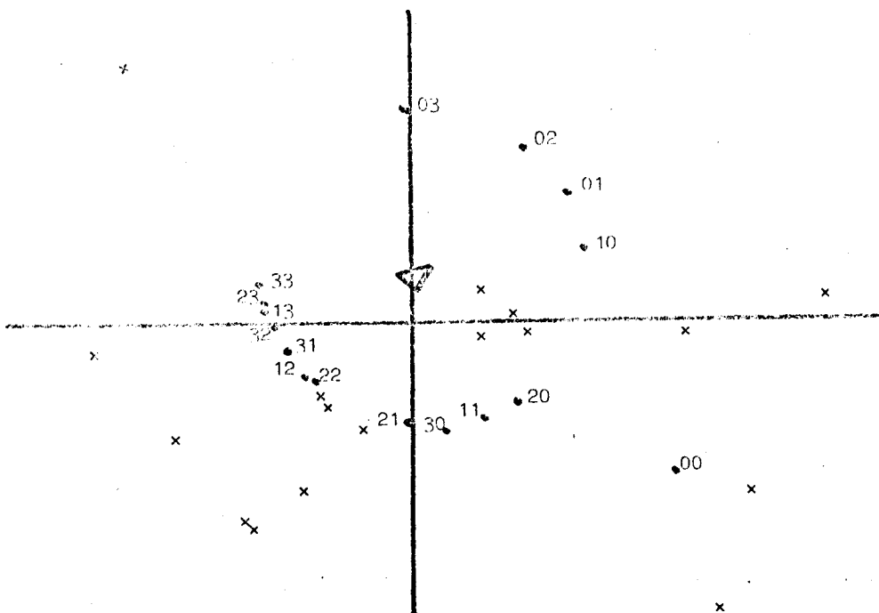
figure 20. Map of family compositions, obtained with the non-metric program MINIRSA.
