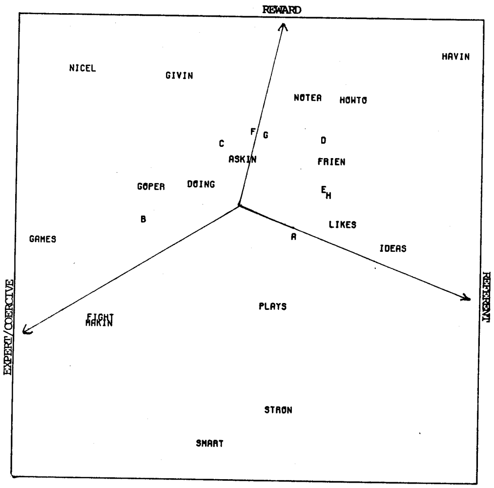
figure 18. Map of power resources (Gold, 1958), obtained with SMACOF-3 (stress = 0.0299).
