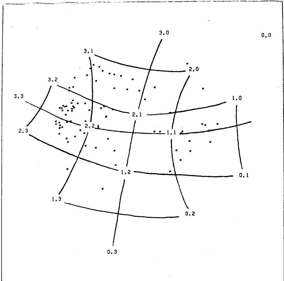
figure 19. Map of family compositions (Delbeke, 1978), obtained with SMACOF-3 (stress = 0.0382).
