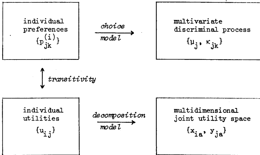
figure 10. The mapping of preference and utility data.
