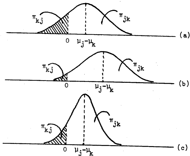
figure 3. Three distributions of utility differences.
