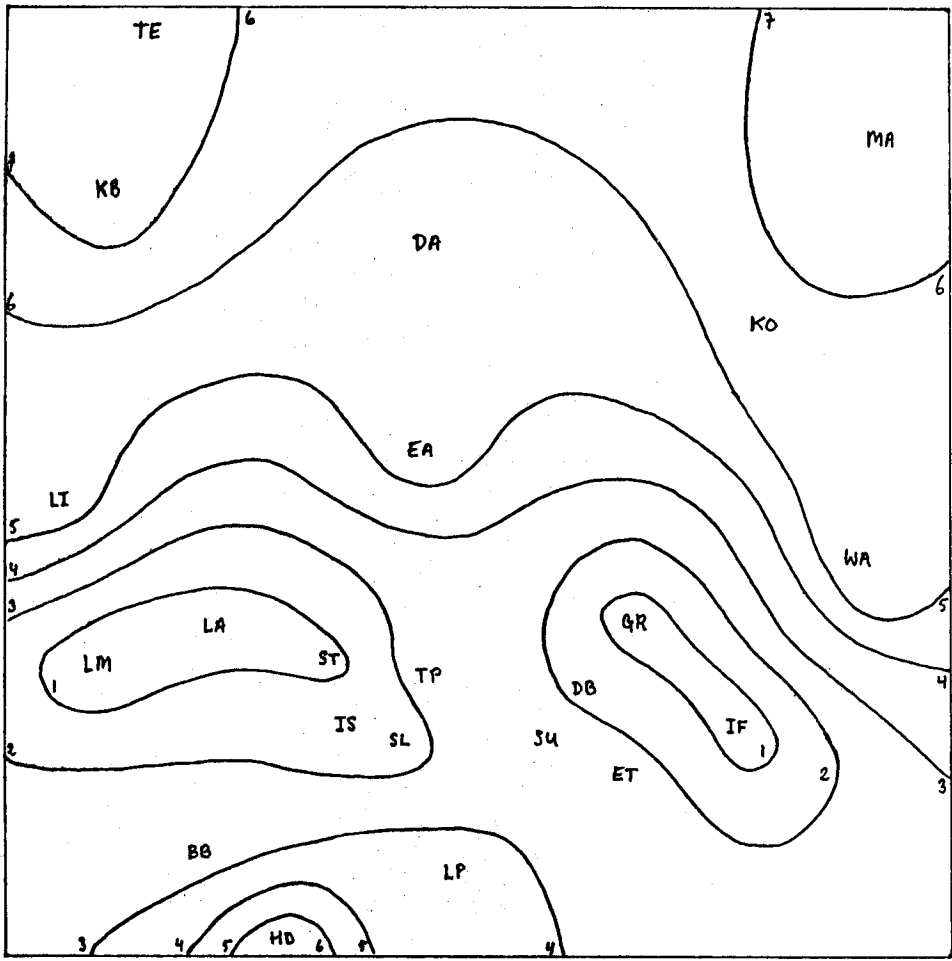
figure 22. Individual cognitive map of educational tasks.
