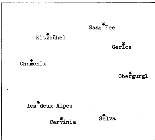
figure 12. Alternative wintersport map showing a circular ordering (circumplex structure).
