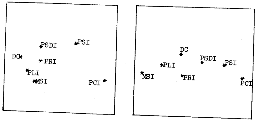
Figure 5. TORSCA structures for standard deviations of utility differences (A) and mean similarity (B) (source: Sjöberg and Capozza, 1975).
