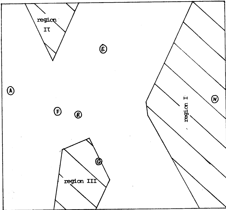
figure 23. Second-grade children's cognitive map of nations with three isotonic regions.
