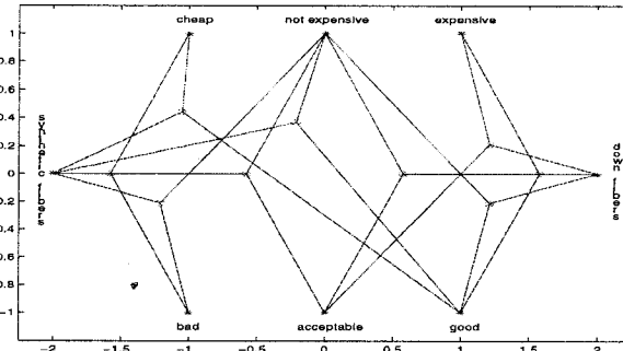
FIGURE 12. Tutte solution with the points of all the variables fixed
