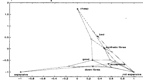
FIGURE 10. Tutte solution with the points of variable Price fixed
