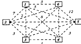
FIGURE 1. The graph representation of a dissimilarity matrix. The numbered squares correspond to the objects, while the weights on certain edges correspond to the dissimilarities
