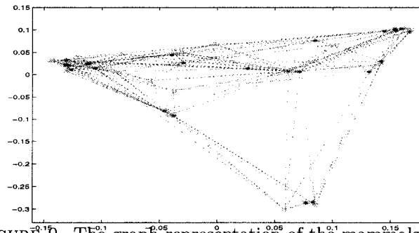
FIGURE 9. The graph representation of the mammals data using the \sigma_{1.6} loss function
