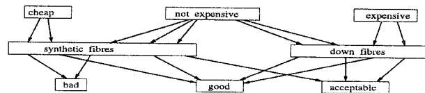
FIGURE 5. A graph drawing of the sleeping bags using Sugiyama's algorithm
