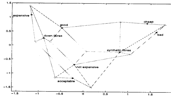
FIGURE 4. The 2-dimensional graph drawing of the sleeping bags using squared Euclidean distances and the X'X = I normalization
