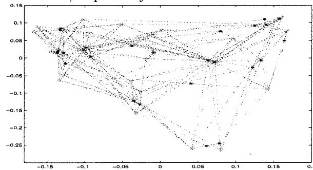
FIGURE 8. The graph representation of the mammals data using the \sigma_2 loss function
