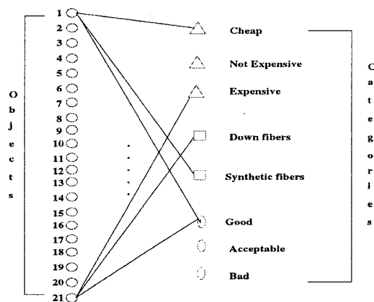
FIGURE 2. The bipartite graph of the sleeping bags example. It can be seen that the first object is cheap, made of synthetic fibres and of good quality, while the last object is expensive, made of down fibres and of good quality
