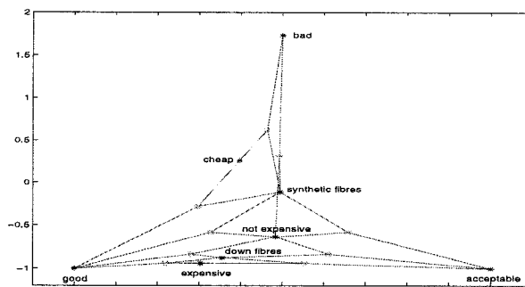
FIGURE 11. Tutte solution with the points of variable Quality fixed
