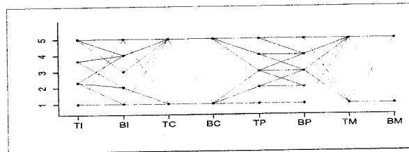
FIGURE 6. Parallel coordinates plot of the mammals data set
