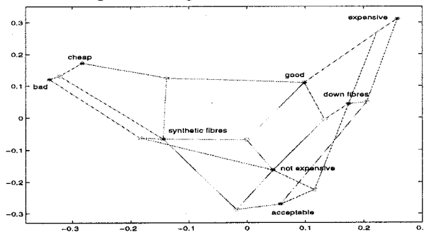
FIGURE 3. The 2-dimensional graph drawing of the sleeping bags using squared Euclidean distances and the Z'Z = I normalization
