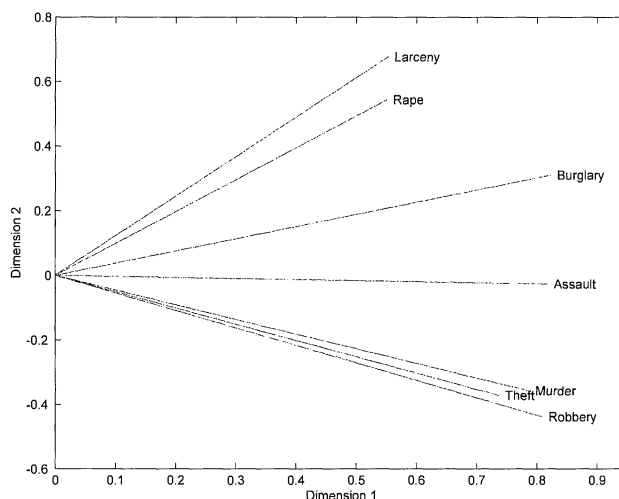
FIG. 10. Component loadings of the seven crime variables.
