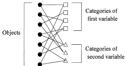
FIG. 1. The bipartite graph of a toy example.
