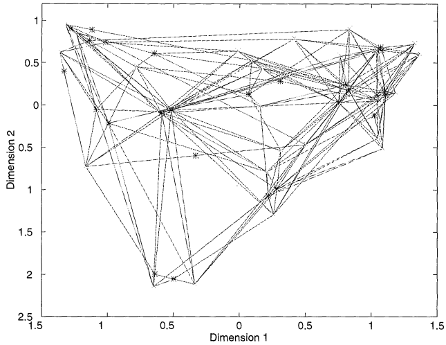
FIG. 4. A two-dimensional graph plot of the mammals data set produced by Homals (x = objects, * = categories).
